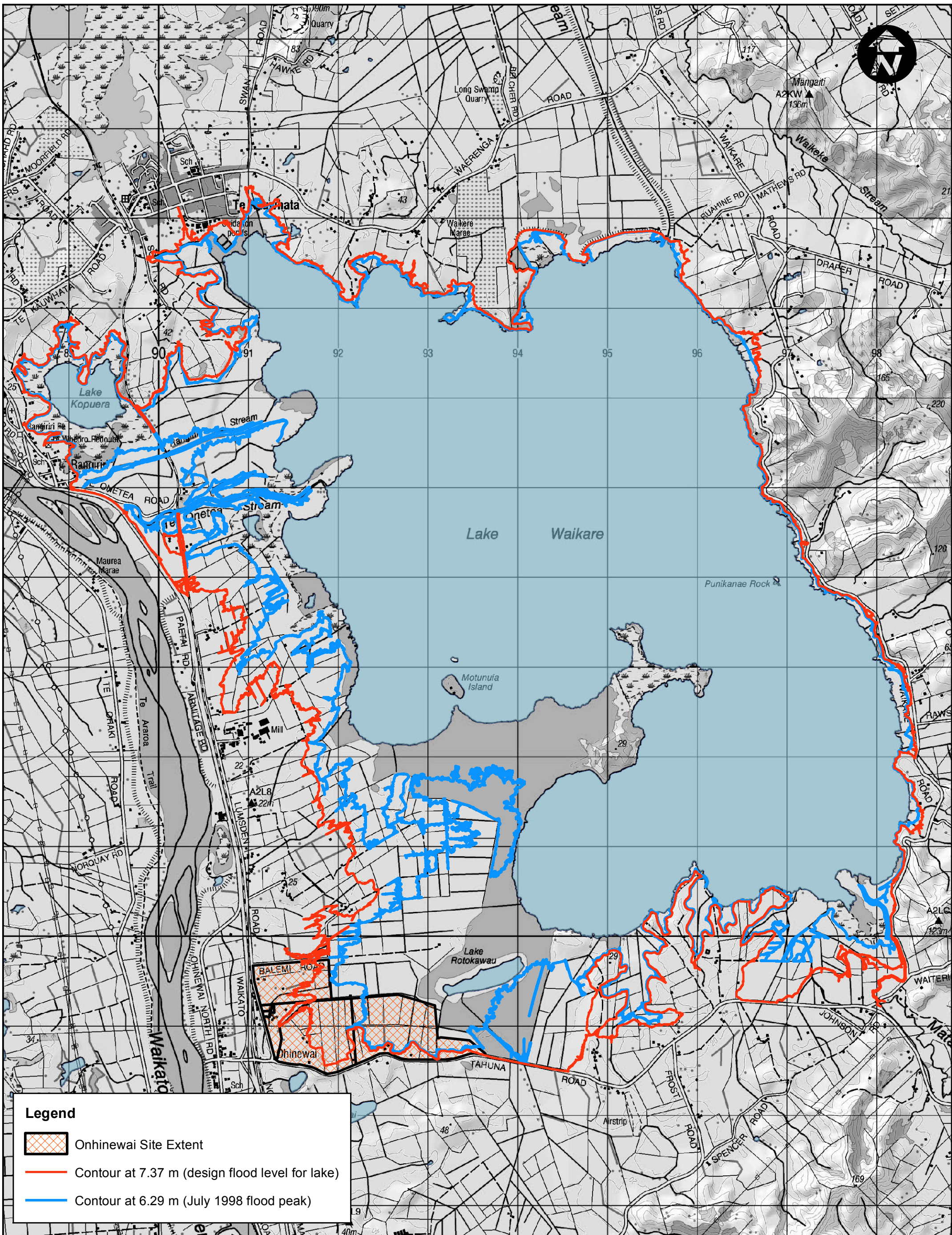
FIGURE 1 Topographic Plan of Land Around Perimeter of Lake Waikare
